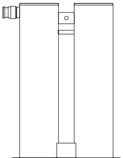
UFV-100H Housing
