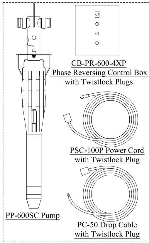
PP-600SC Pump
